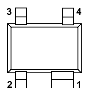
Top view MSB842
